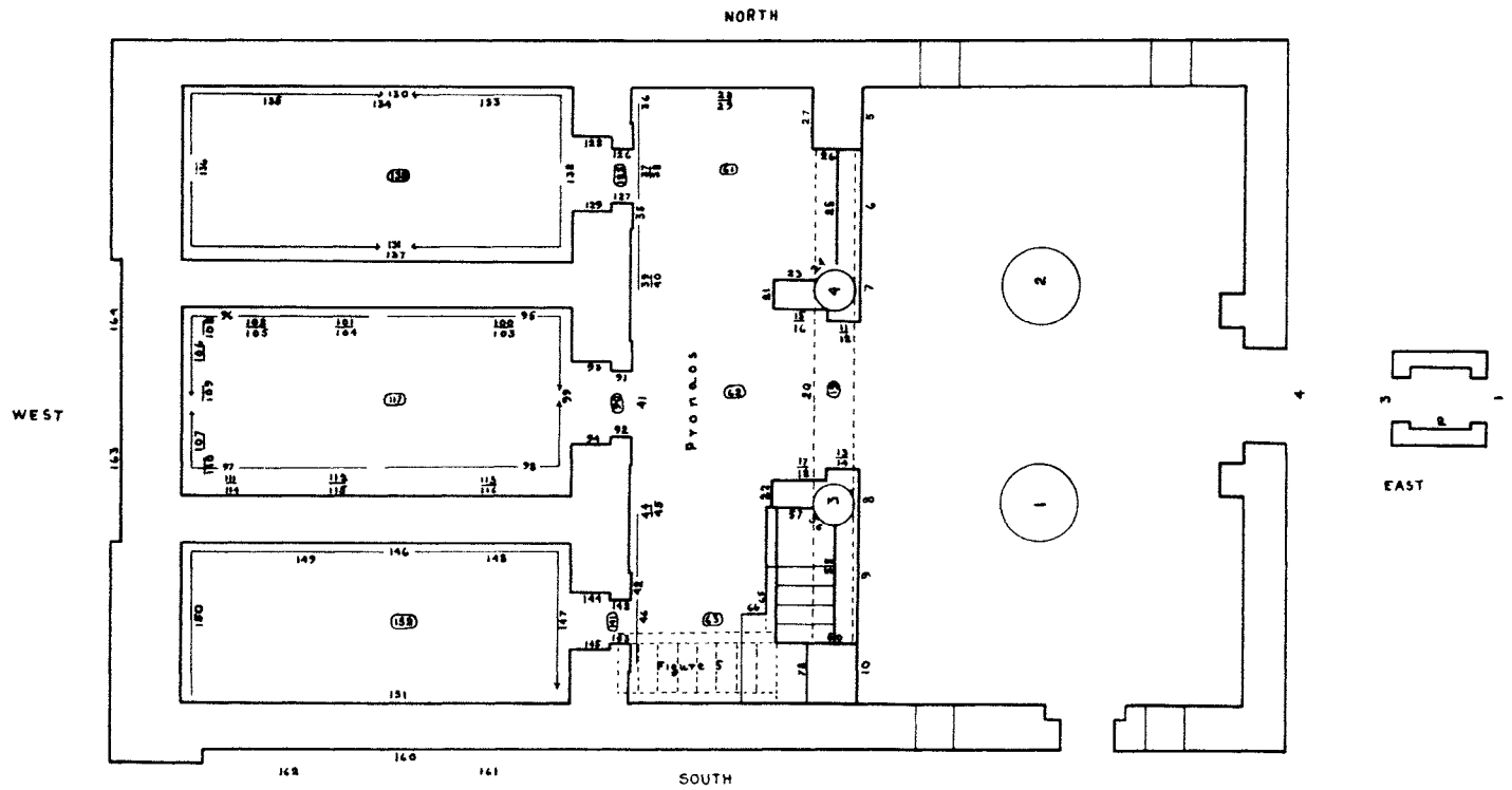
Fig. 4. Ground Plan
